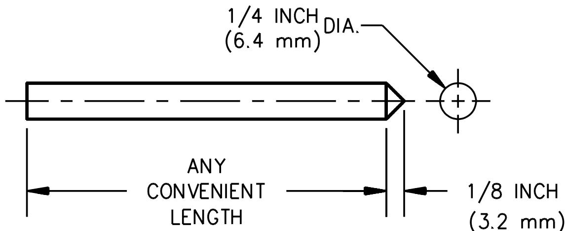
Figure 64.1 Probe for hand-supported enclosure
