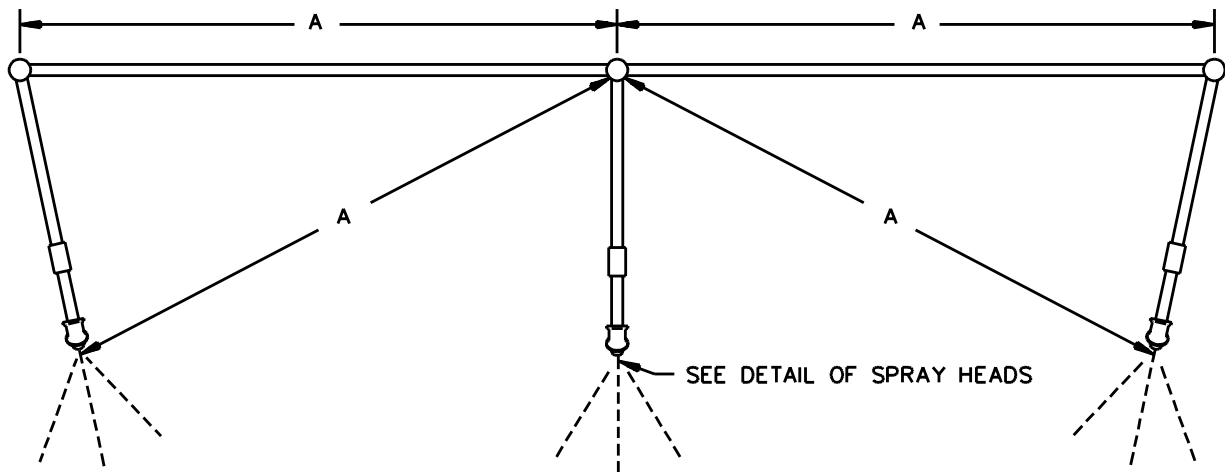
Figure 65.2 Water-spray piping PLAN VIEW
