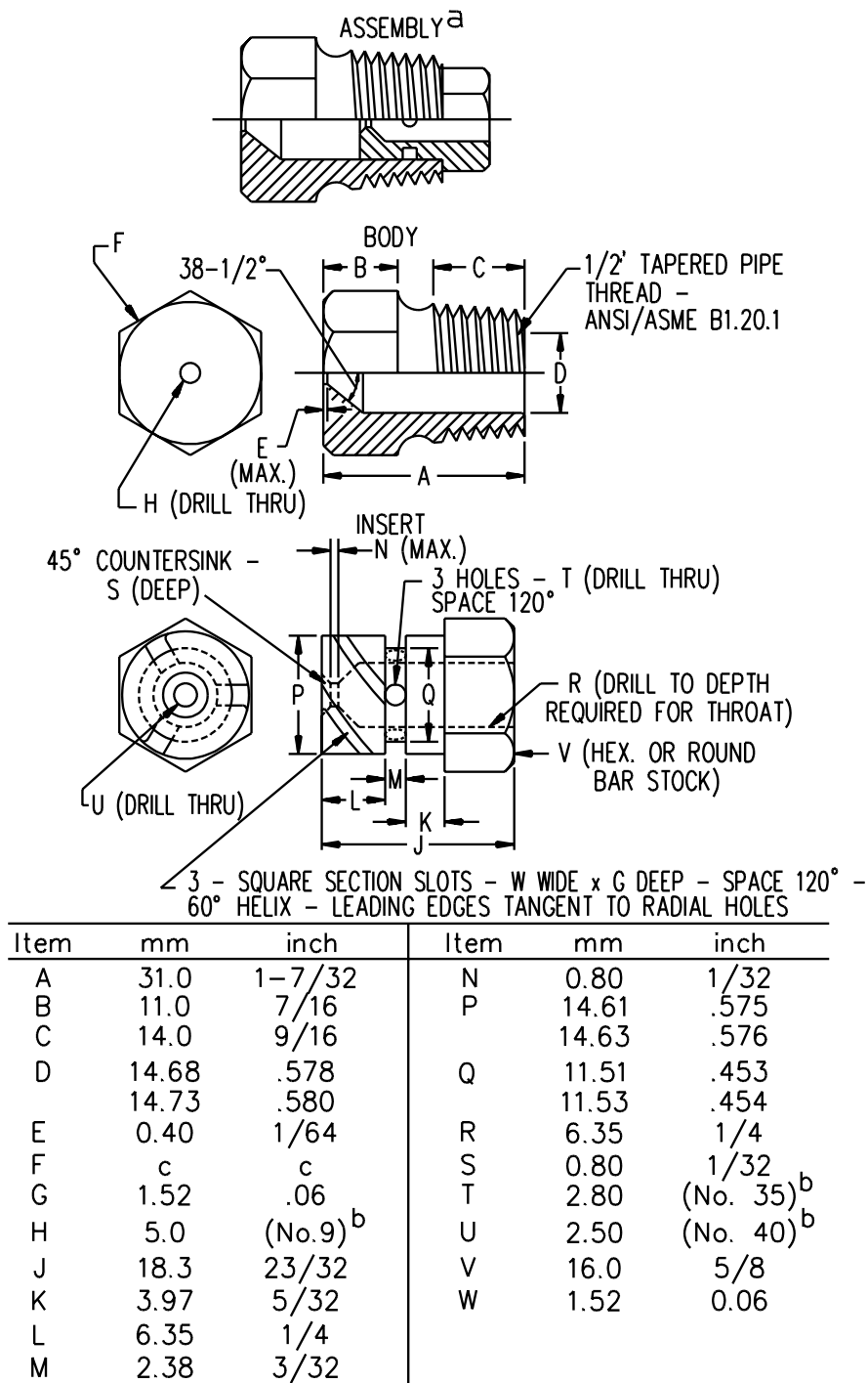
Figure 65.1 Spray head
