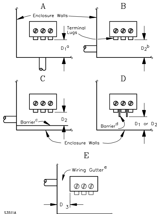
Figure 19.1 Wire bending space
